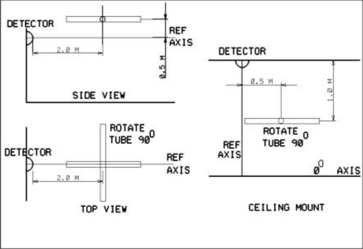
Figure K.1 - Immunity to fluorescent lamp interference
