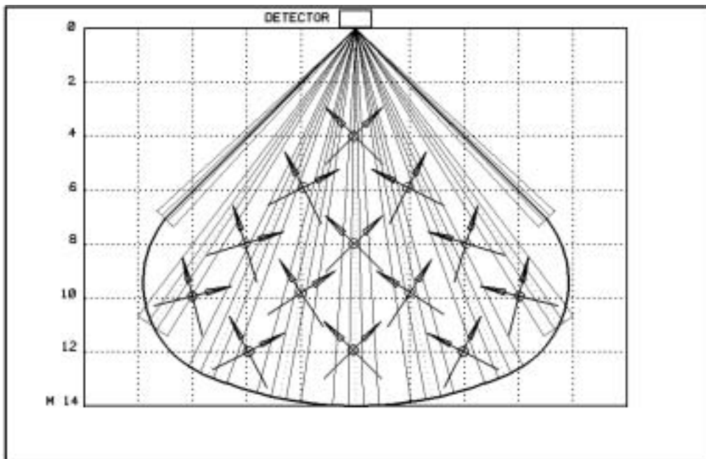
Figure C.2 – Detection within the boundary, & effect of control adjustments
