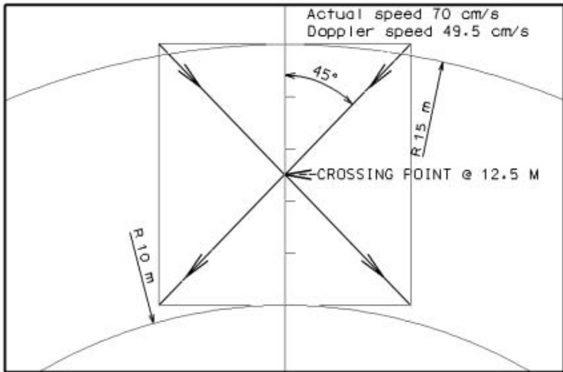
Figure G.1 - Calibration of microwave SWT
