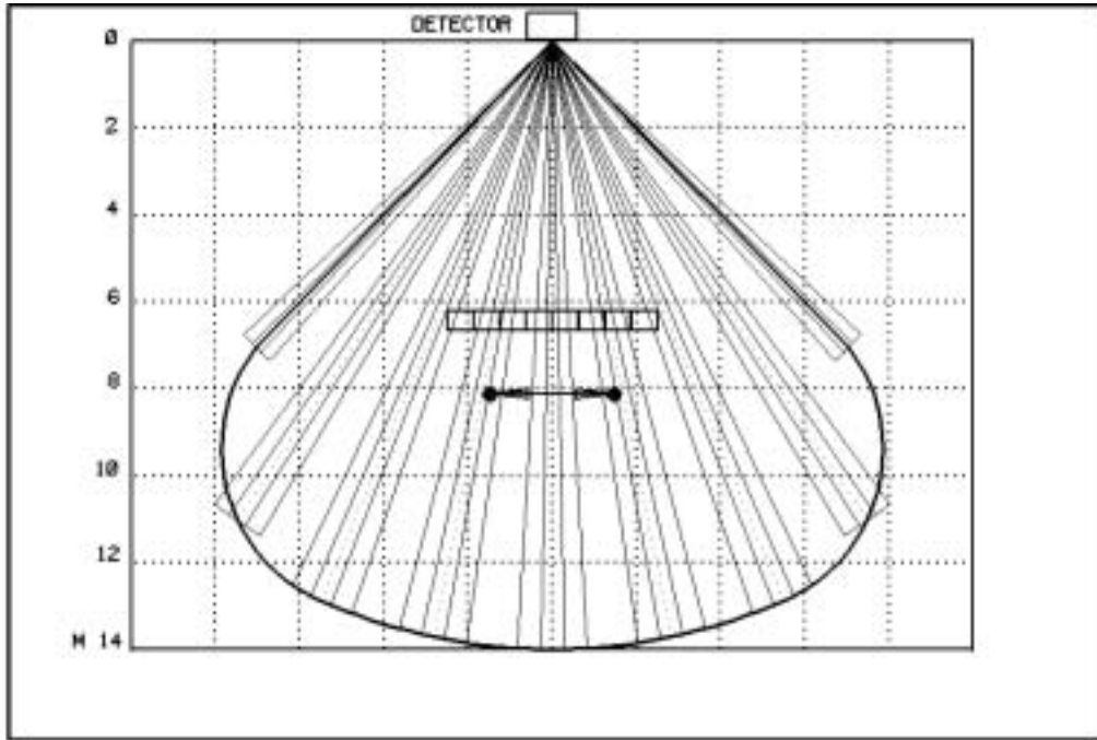
Figure C.5 - Significant range reduction
