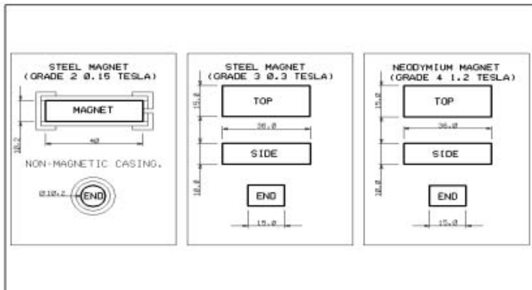
Figure A.1 - Format of standard test magnets
