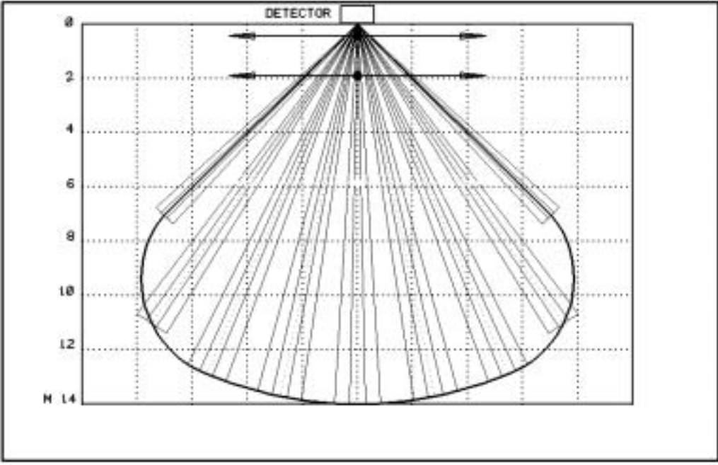
Figure C.4 - Close-in detection
