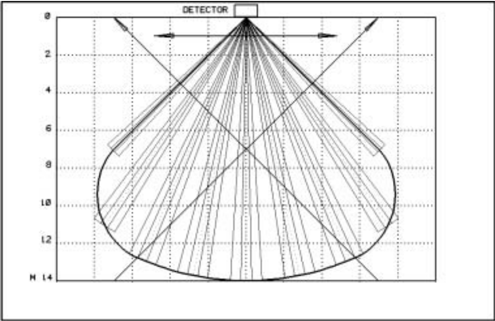
Figure C.3 - High velocity and intermittent movement
