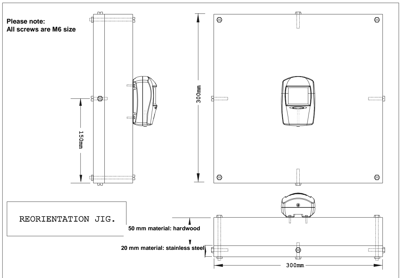
Figure M.1 - Re-orientation test
