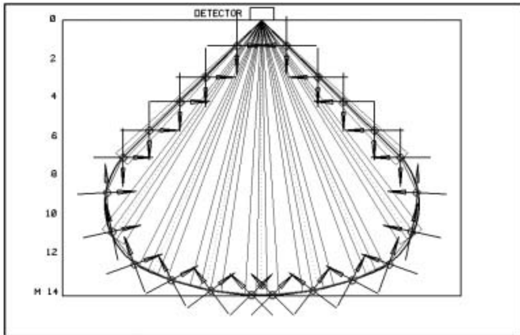
Figure C.1 – Detection across the boundary, & effect of control adjustments
